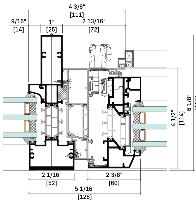
S 155 FRAME + CASEMENT
