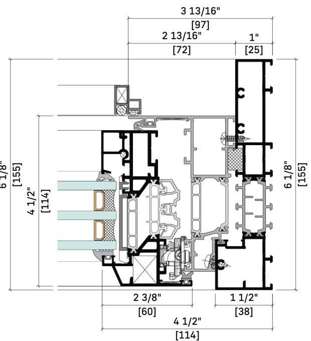
S 155 FRAME + CASEMENT
