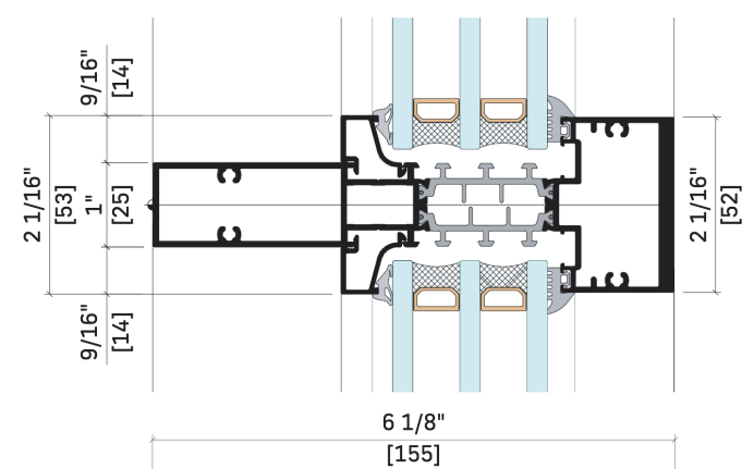
VERTICAL S 155 MULLION
