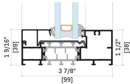
S 100 FRAME
