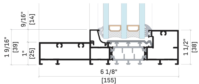
S 155 FRAME
