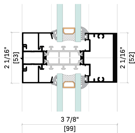
VERTICAL S 100 MULLION
